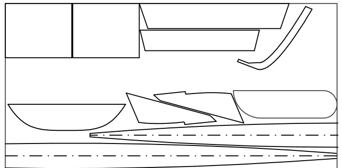
3/4" PLYWOOD PANEL LAYOUTS
