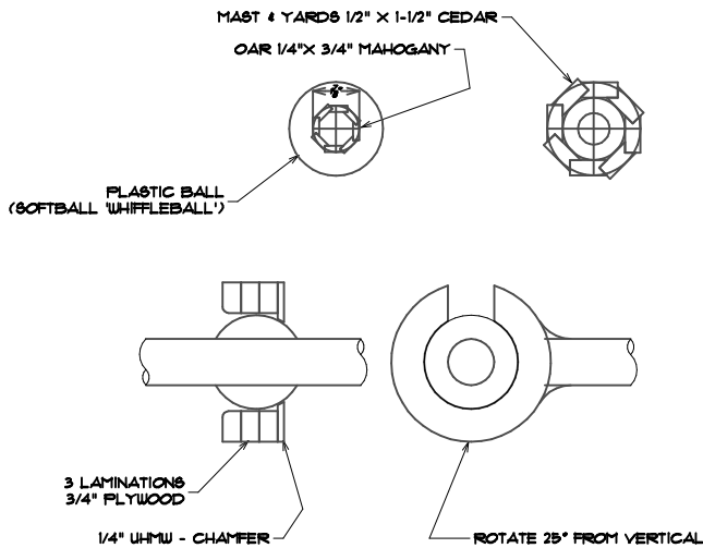
BIRDMOUTH BITS
