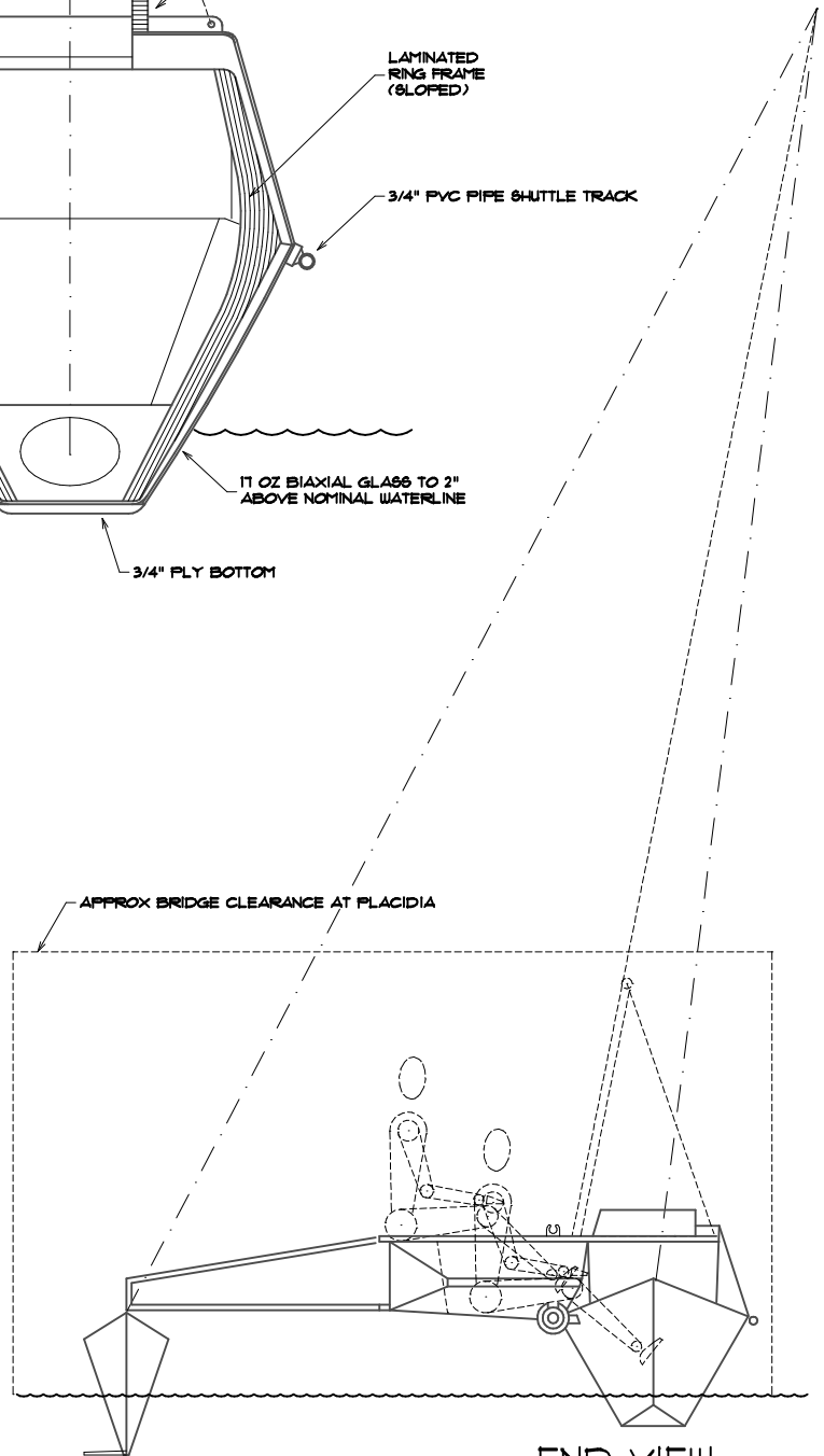
END VIEW
