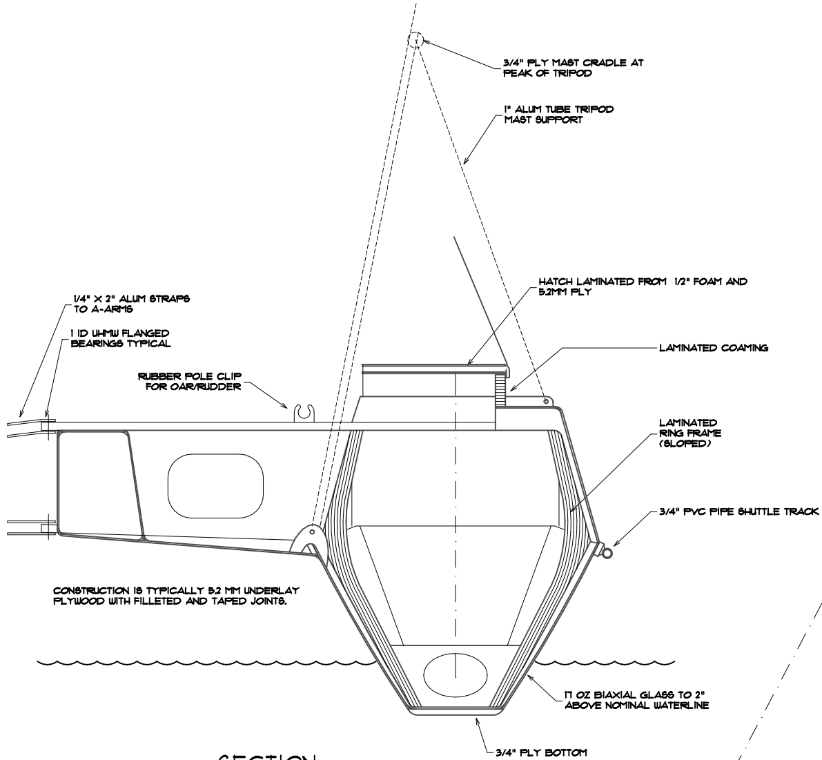
SECTION
